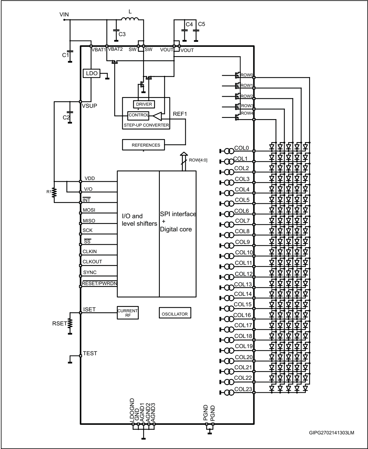
Figure 1. Application schematic
