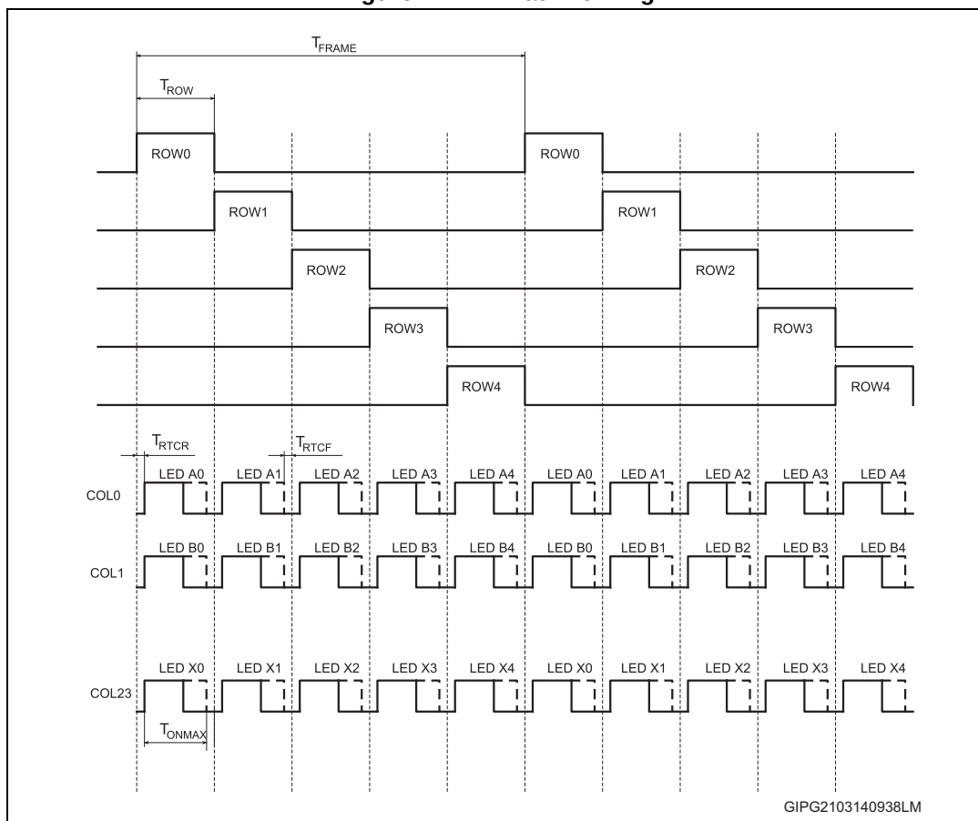
Figure 4. LED matrix timing
