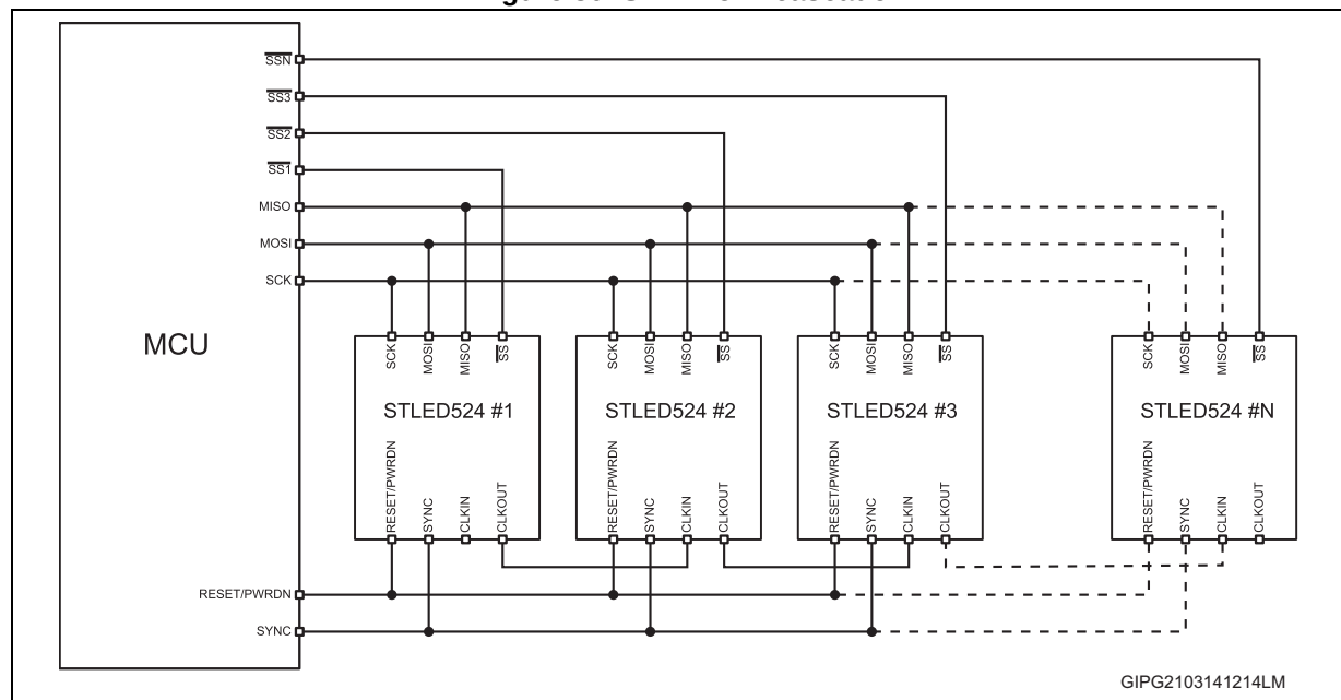
Figure 30. STLED524 cascade
