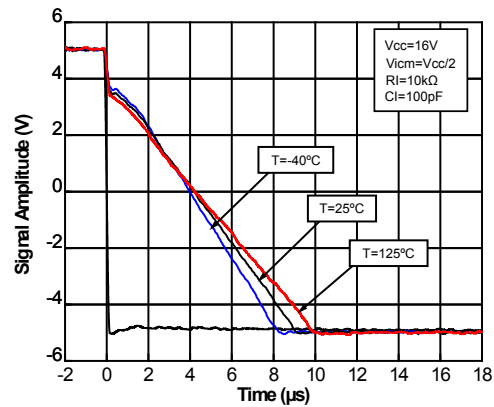
Figure 18. Negative slew rate at V_{CC} = 16\text{ V}
