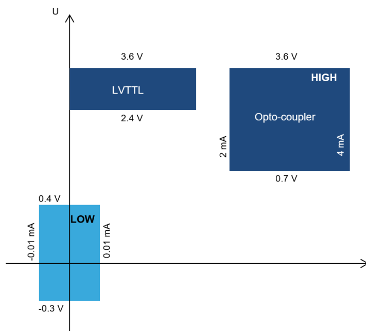
Figure 5. Output U-I operation
