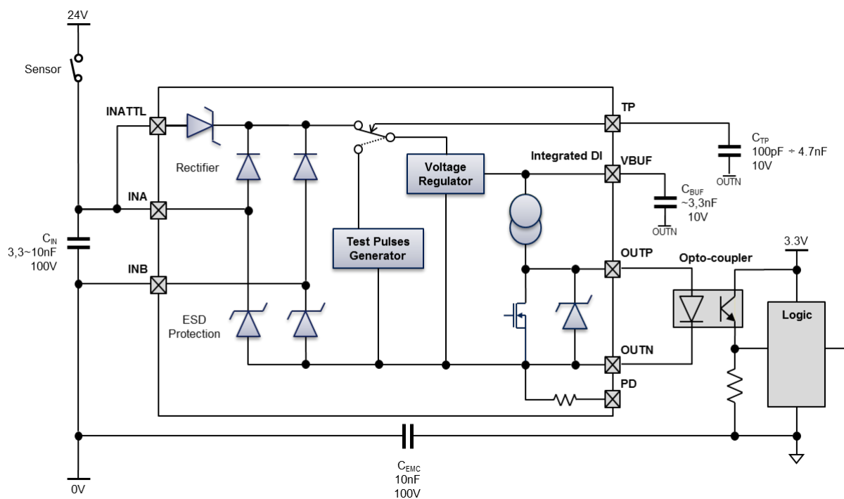
Figure 9. High side - isolated configuration - test pulse activated
