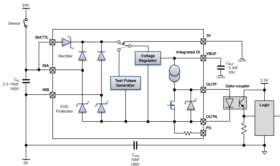
Figure 11. High side - isolated configuration - test pulse not activated
