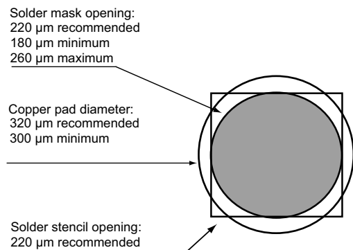
Figure 16. Footprint - 3 mils stencil - solder mask defined
