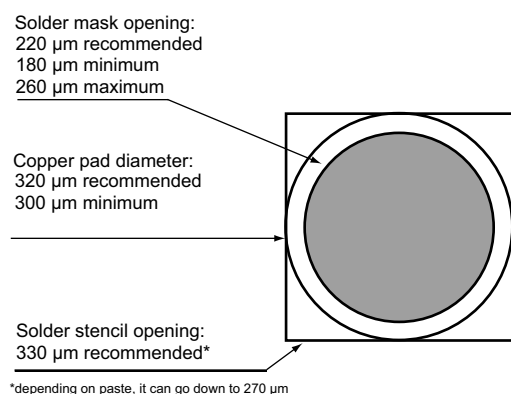
Figure 18. Footprint - 5 mils stencil - solder mask defined
