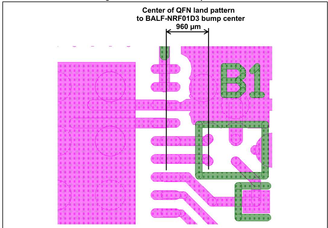
Figure 12. BALF-NRF01D3 position
