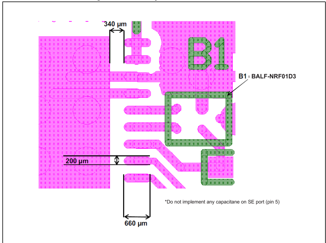
Figure 12. BALF-NRF01D3 position
