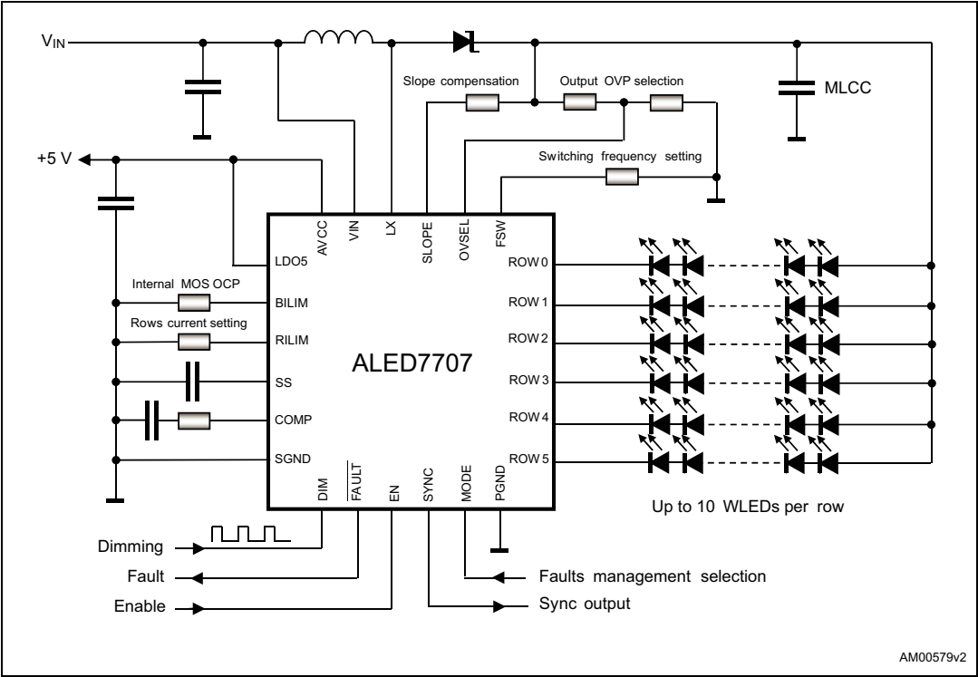
Figure 1. Application circuit
