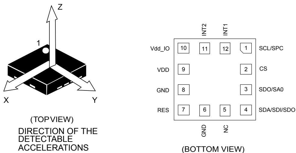
Figure 2. Pin connections
