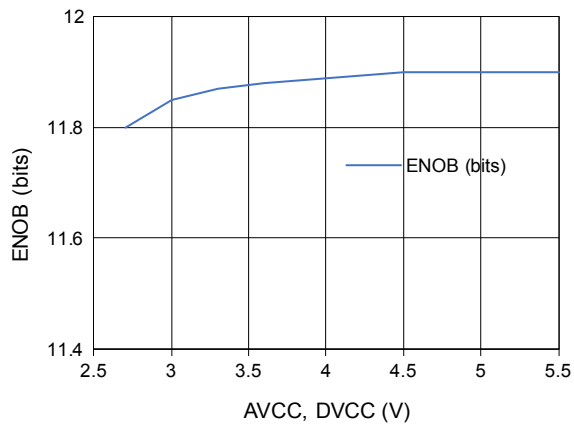
Figure 14. ENOB vs. AVCC = DVCC
