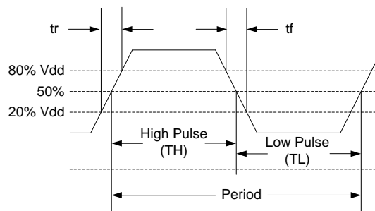
Figure 4. Waveform [4]
