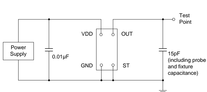
Figure 3. Test Circuit
