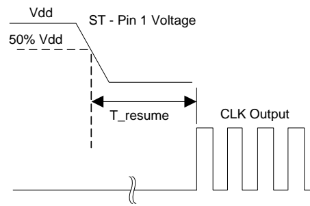
Figure 6. Resume Timing [5,6]
