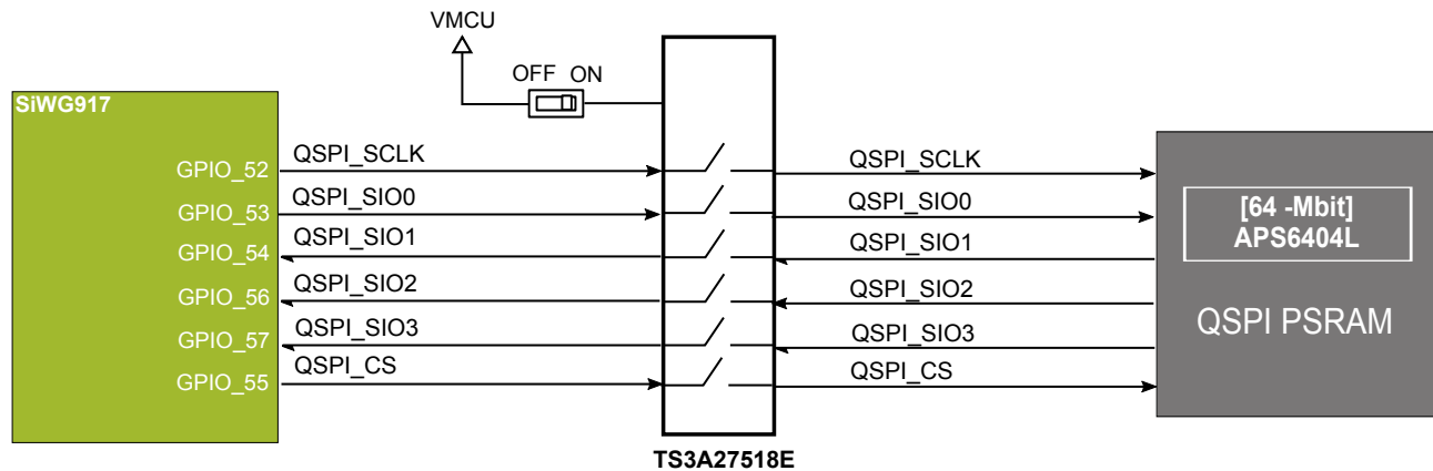
Figure 3.9. QSPI PSRAM
