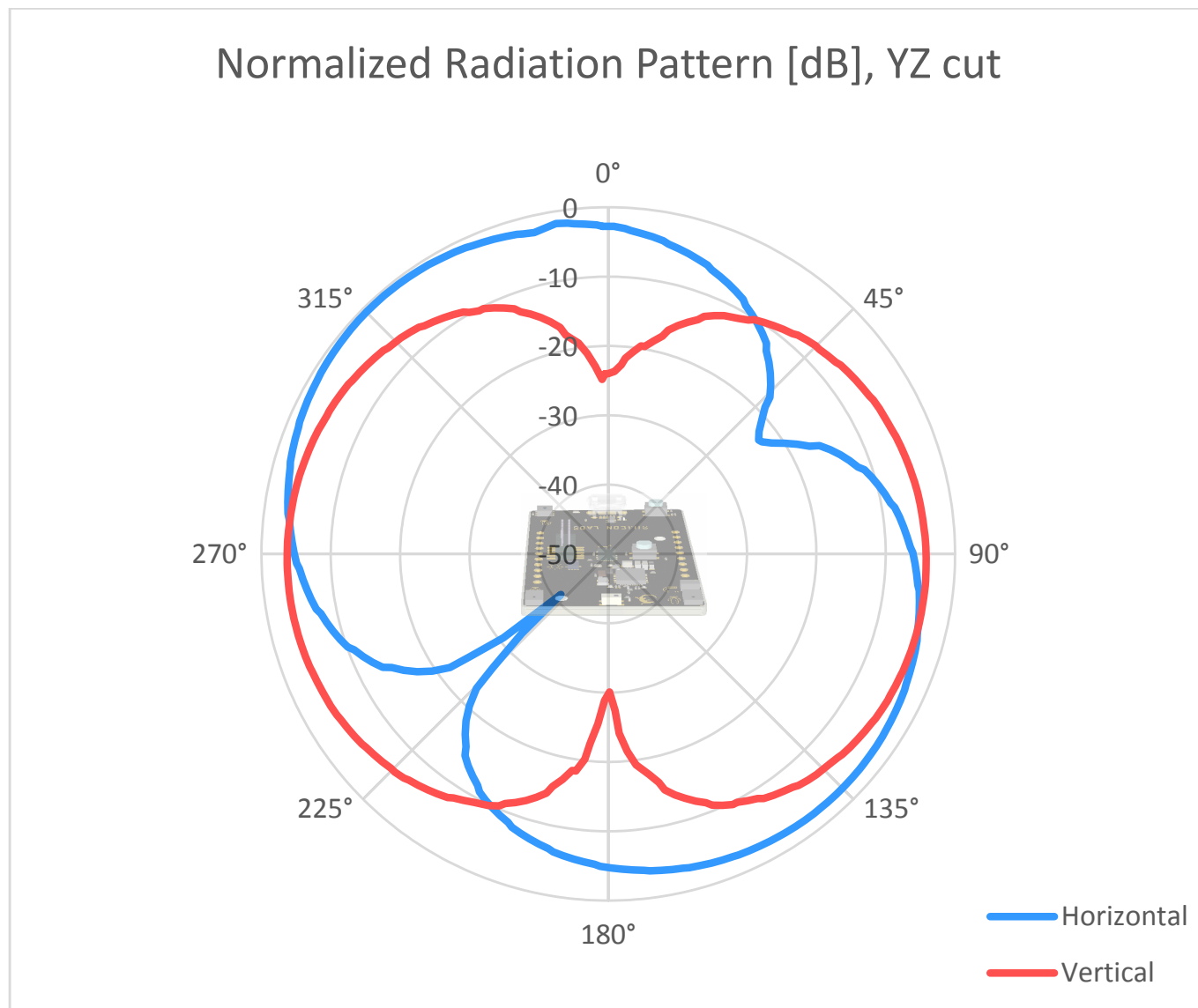
Figure 5.7. Antenna Pattern - YZ
