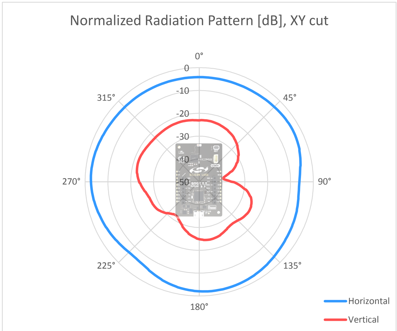
Figure 5.5. Antenna Pattern - XY
