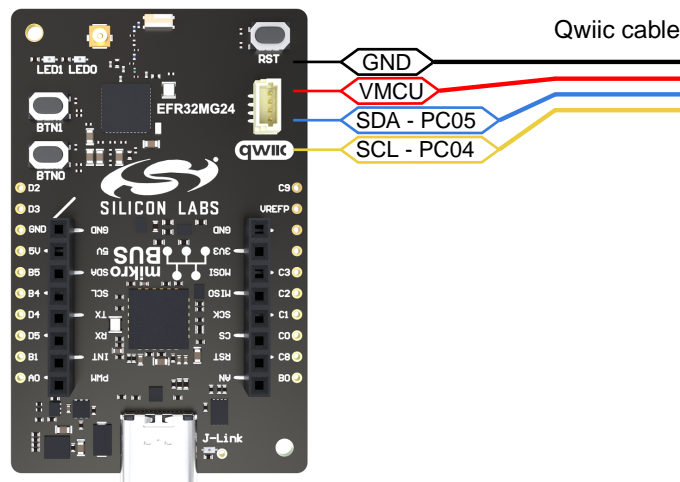
Figure 3.7. Qwiic Connector
