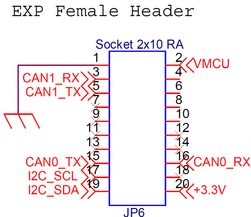
Figure 2.4. Isolated CAN EXP Receptacle Header
