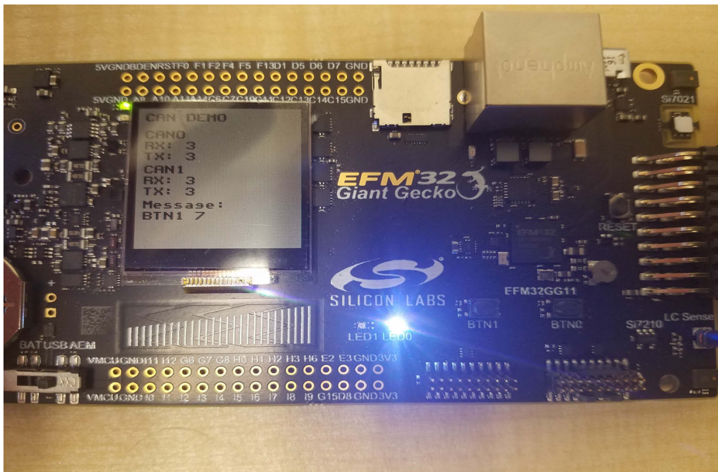
Figure 3.8. CAN Example Screen
