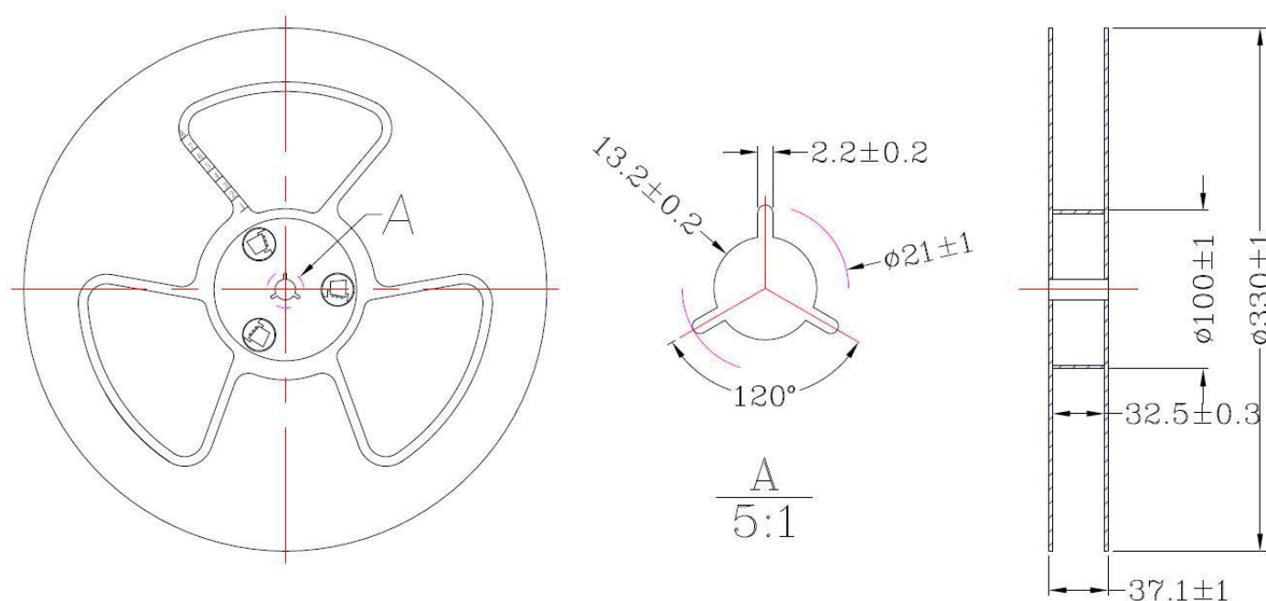
Figure 10.2. Reel Dimensions
