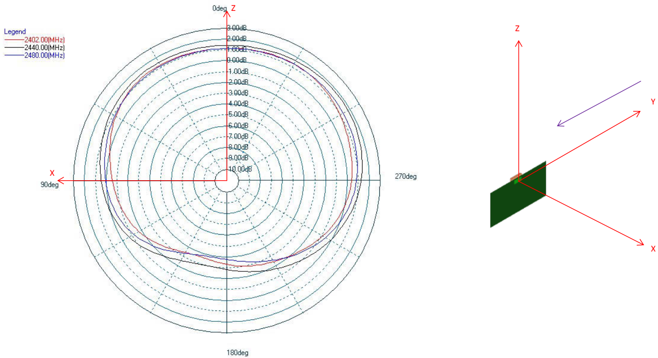
Figure 4.1. Typical 2D Antenna Radiation Patterns - \Phi = 0^\circ (Side View) Gain (dBi)
