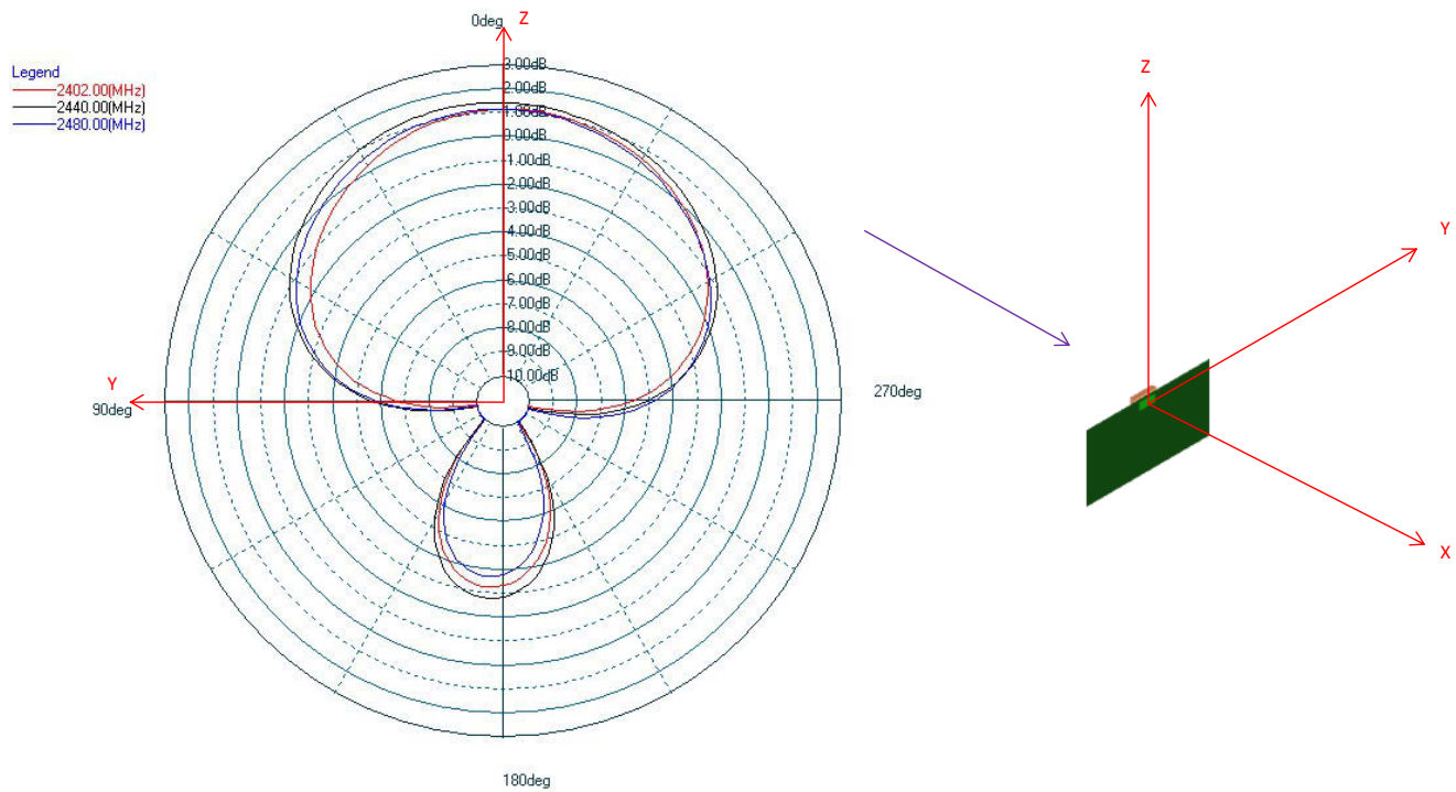
Figure 4.2. Typical 2D Antenna Radiation Patterns - \Phi = 90^\circ (Top View) Gain (dBi)
