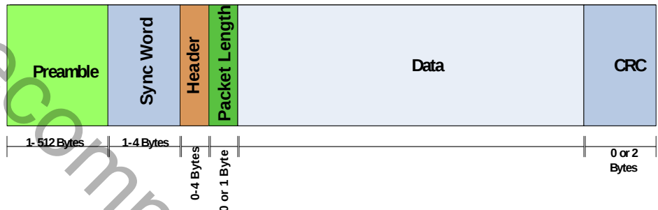
Figure 11. Packet Structure
