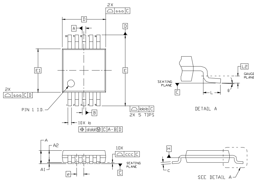
Figure 9. 10-Pin MSOP Package
