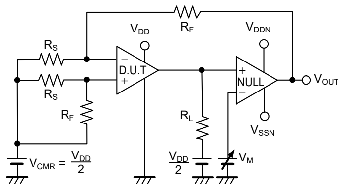
Figure 10 Test Circuit 8
