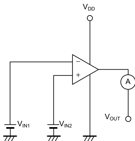
Figure 8 Test Circuit 6
