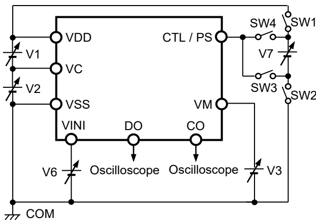
Figure 9 Test Circuit 5
