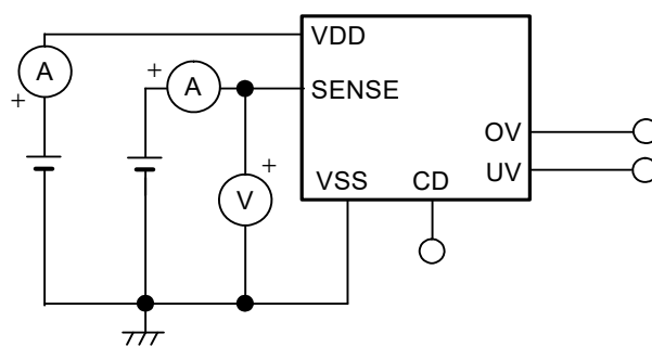
Figure 8 Test Circuit 4
