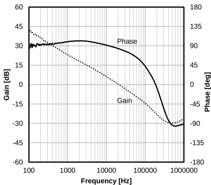
Figure 38. Frequency Characteristic ( V_{VIN} = 13\text{ V} , T_a = 25\text{ }^{\circ}\text{C} , I_{OUT} = 1.0\text{ A} )
