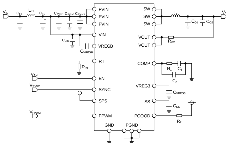
Reference Circuit
