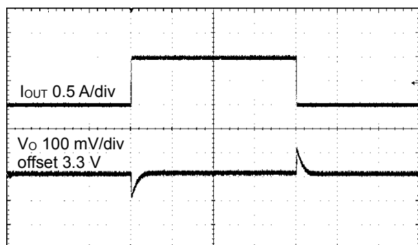
Figure 40. Load Response 1 ( V_{IN} = 13\text{ V} , T_a = 25\text{ }^{\circ}\text{C} , FPWM = H, I_{OUT} = 10\text{ mA} to 1.0\text{ A} , 1\text{ ms/div} )
