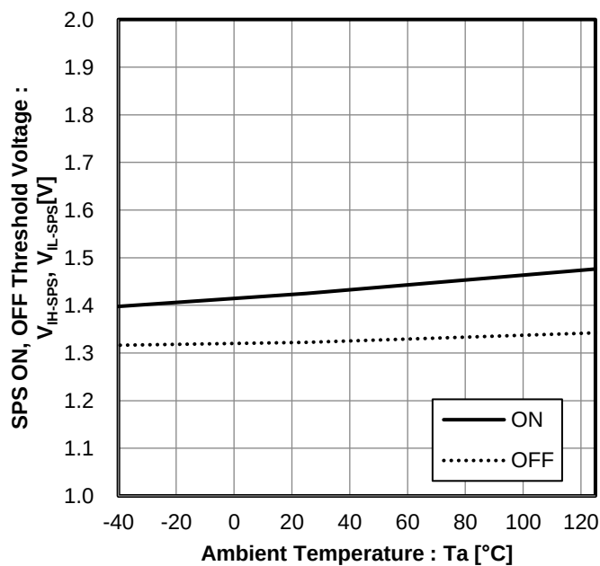
Figure 16. SPS ON/OFF Threshold Voltage vs Ambient Temperature
