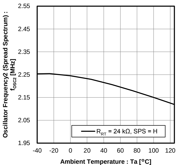
Figure 10. Oscillator Frequency2 (Spread Spectrum) vs Ambient Temperature
