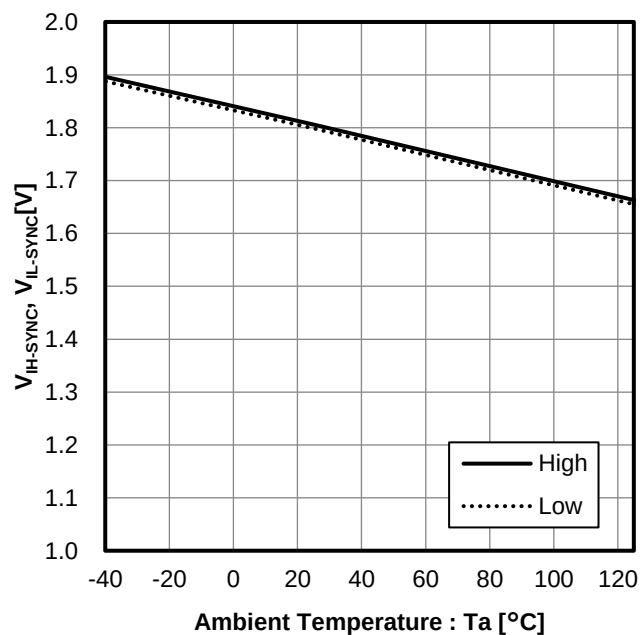
Figure 12. SYNC High/Low Threshold Voltage vs Ambient Temperature
