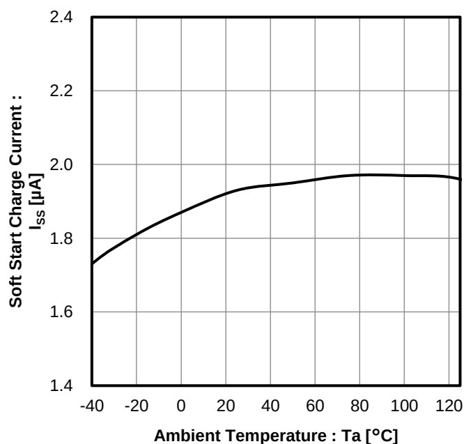
Figure 18. Soft Start Charge Current vs Ambient Temperature
