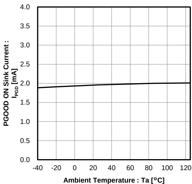
Figure 22. PGOOD ON Sink Current vs Ambient Temperature
