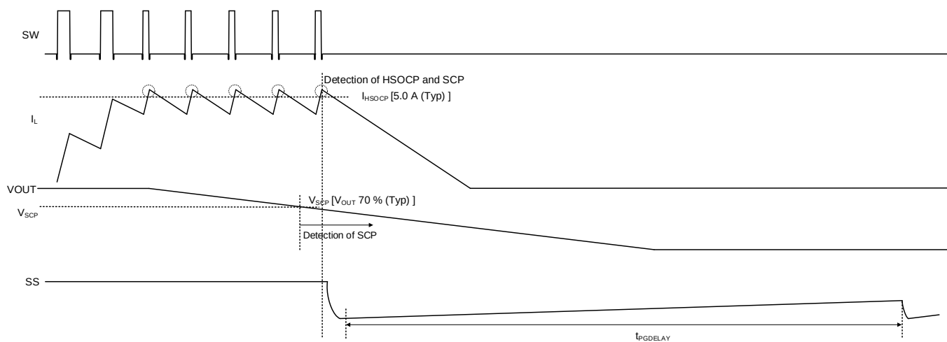
Case4: Detecting peak current limit when SCP is detected
