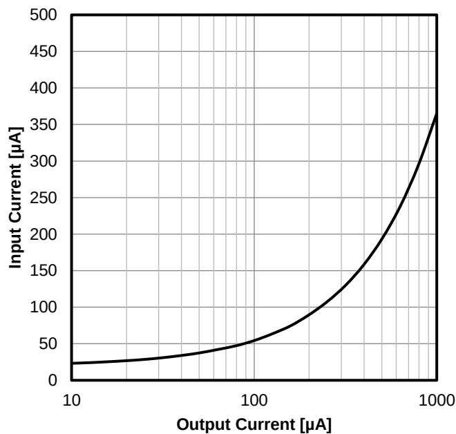
Figure 37. Input Current vs Output Current ( V_{VIN} = 13\text{ V} , T_a = 25\text{ }^{\circ}\text{C} , LLM)
