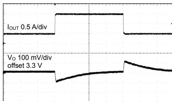
Figure 41. Load Response 2 ( V_{IN} = 13\text{ V} , T_a = 25\text{ }^{\circ}\text{C} , FPWM = H, I_{OUT} = 0.5\text{ A} to 1.5\text{ A} , 100\text{ }\mu\text{s/div} )
