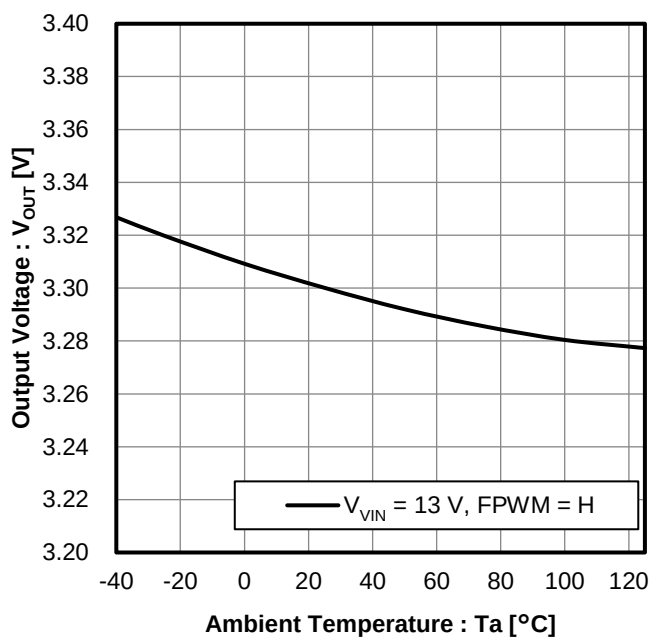
Figure 5. Output Voltage vs Ambient Temperature
