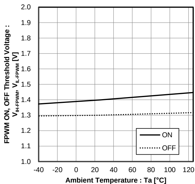
Figure 14. FPWM ON/OFF Threshold Voltage vs Ambient Temperature
