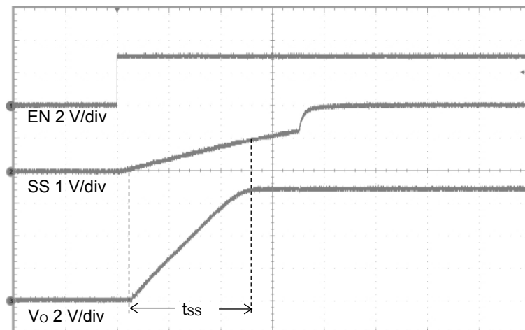
Figure 35. Soft start waveform ( V_{IN} = 13 \text{ V} , C_{SS} = 0.01 \mu\text{F} , 2 ms/div)
