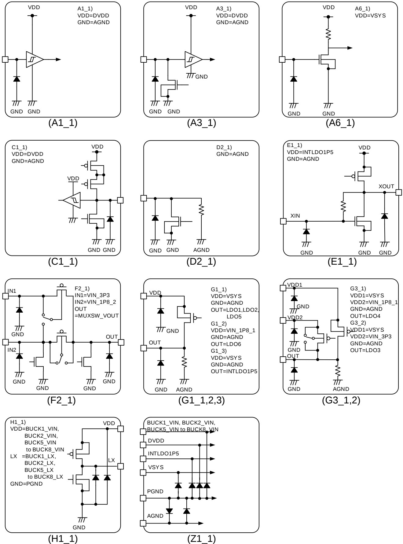
Figure 1-4. I/O Equivalence Circuit 1
