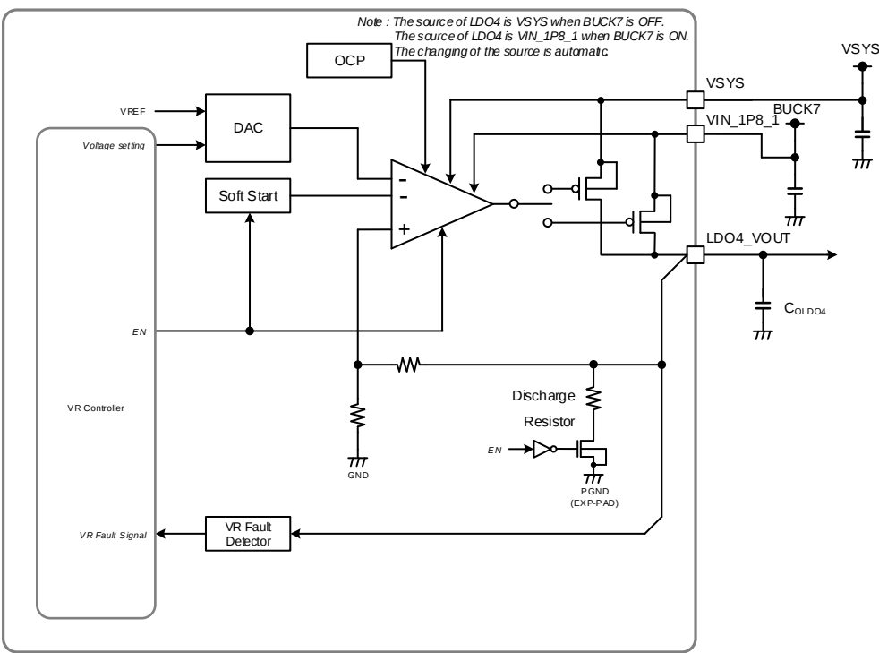
Figure 5-11. LDO4 Block Diagram
