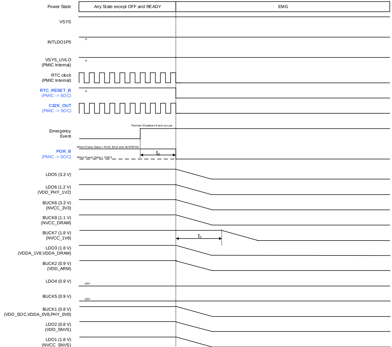
Figure 3-29. Emergency Shutdown
