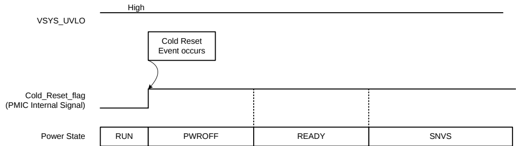
Figure 3-8. Cold Reset Condition for moving to SNVS
