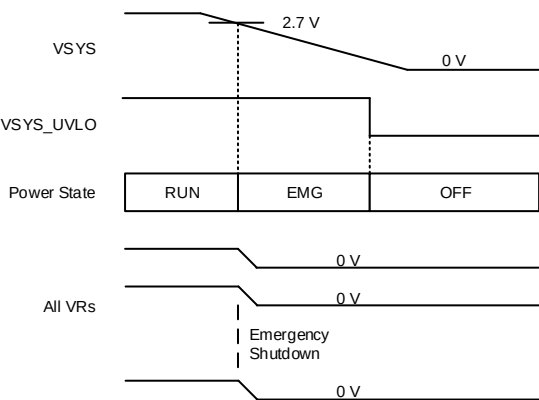
Figure 3-15. EMG to OFF Power State Transition
