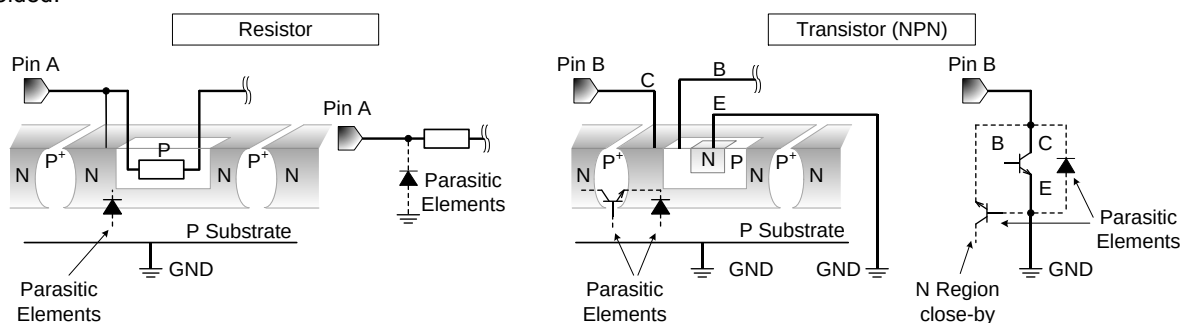
Figure 7-1. Example of Monolithic IC Structure
