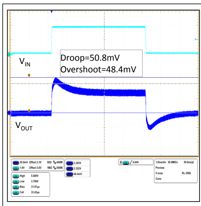
Figure 34. Line Transient Response ( V_{IN}=3.7\text{V} \leftrightarrow 5.5\text{V} , t_r=t_f=30\mu\text{s} , V_{OUT}=3.3\text{V} , I_{OUT}=500\text{mA} )
