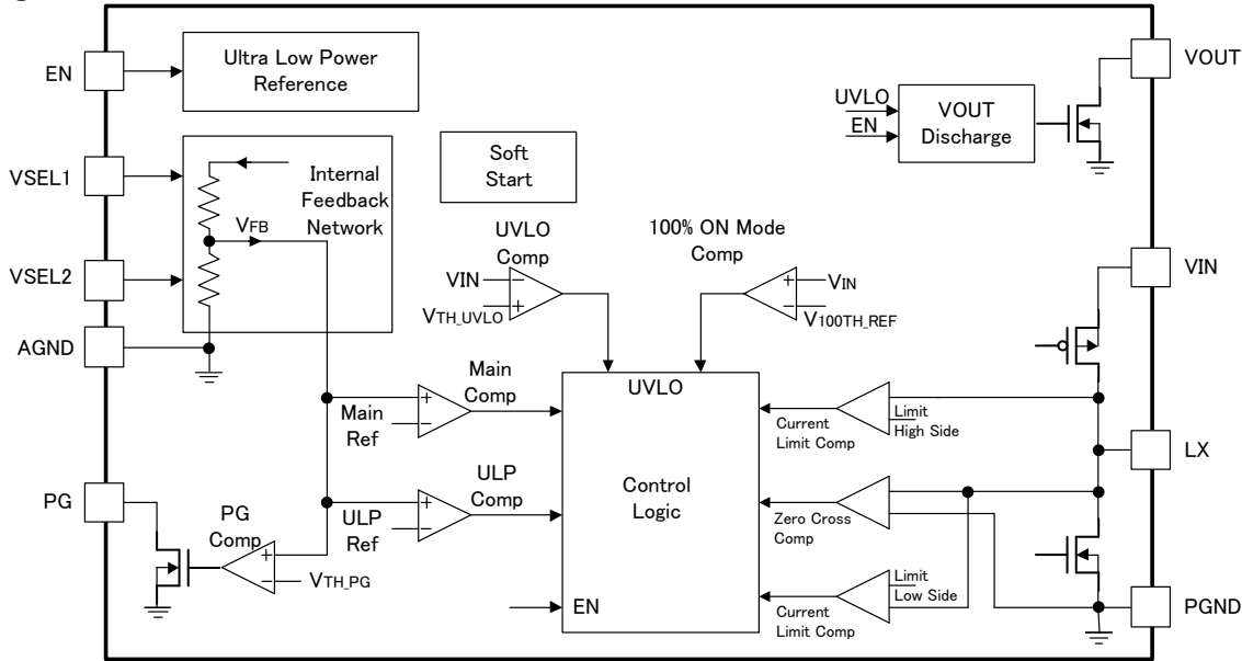
Figure 3. Block Diagram
