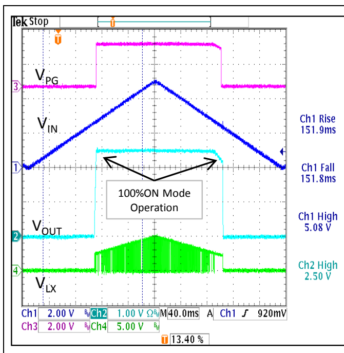
Figure 41. Input Voltage Ramp Up/Down ( V_{IN}=0\text{V}\leftrightarrow 5.0\text{V} , V_{OUT}=2.5\text{V} , I_{OUT}=500\text{mA} , PG=V_{OUT} )
