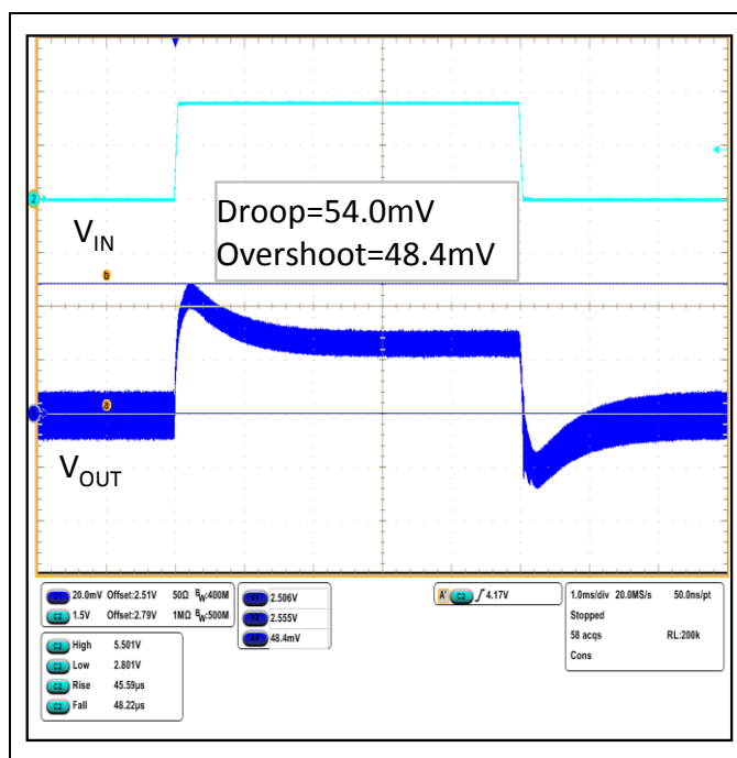
Figure 32. Line Transient Response ( V_{IN}=2.8\text{V} \leftrightarrow 5.5\text{V} , t_r=t_f=45\mu\text{s} , V_{OUT}=2.5\text{V} , I_{OUT}=500\text{mA} )
