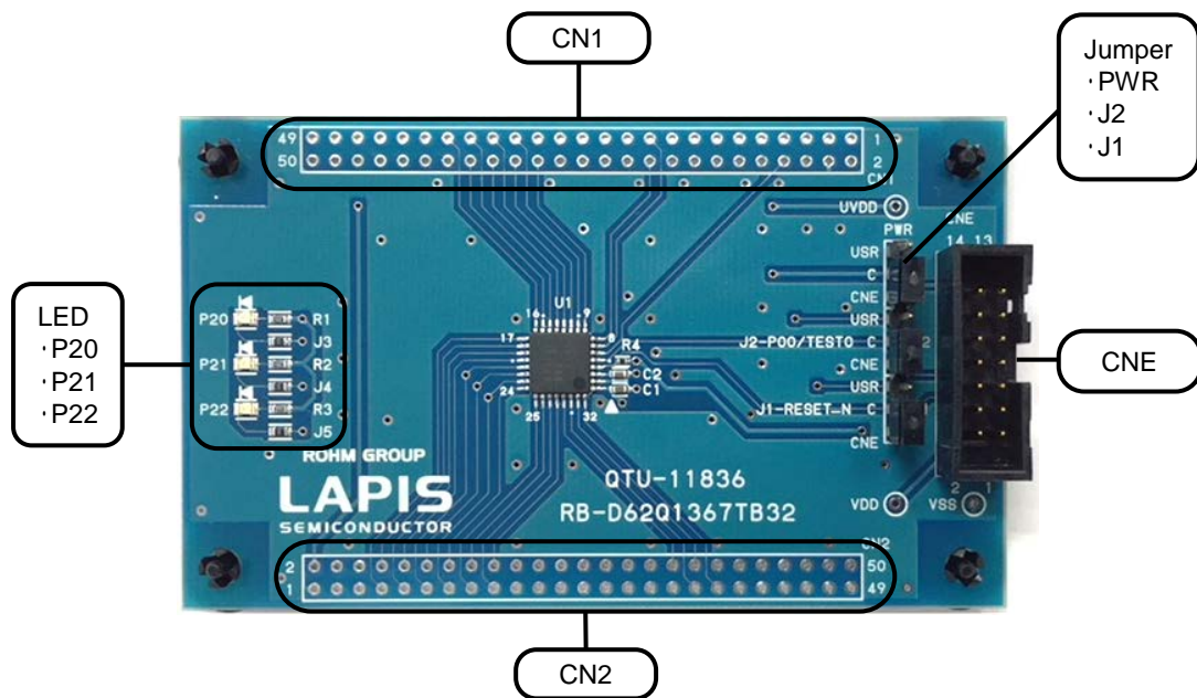
Fig. 1 ML62Q1367 Reference Board Outline Diagram
