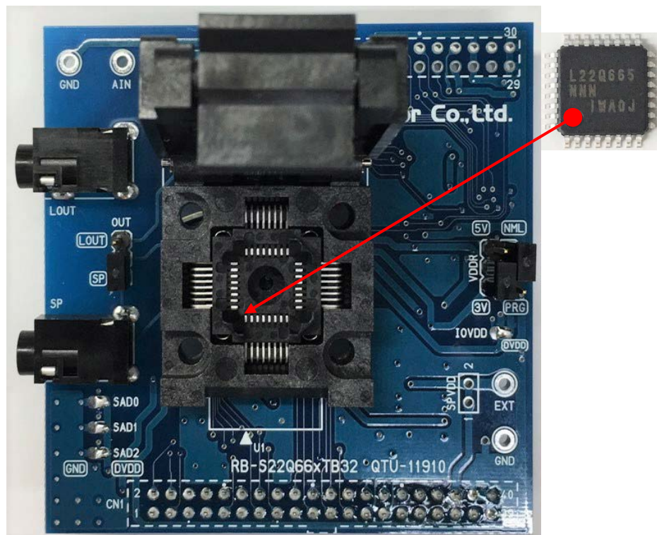
Figure 1 Outline Diagram
