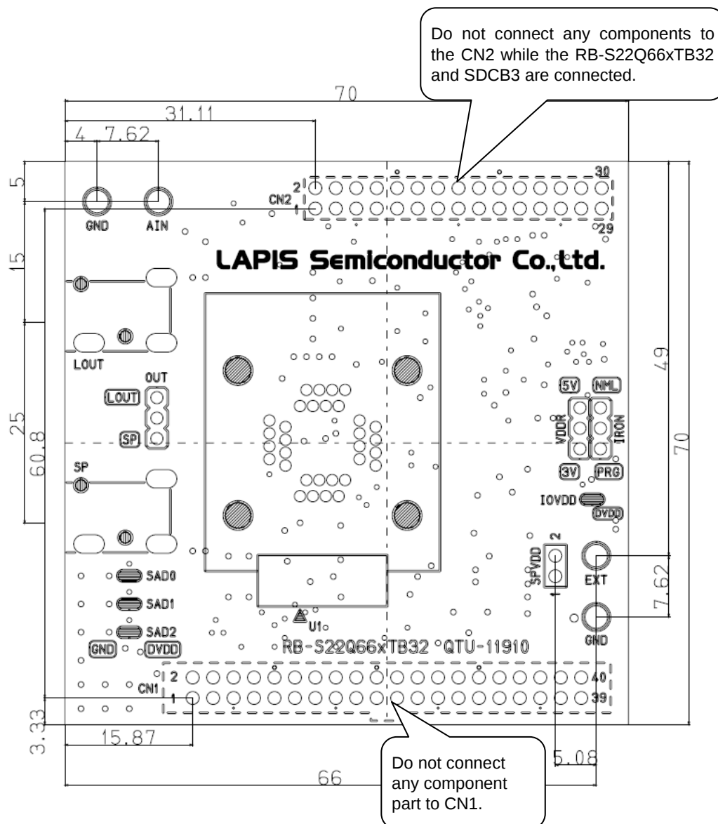
Figure 2 PCB layout
