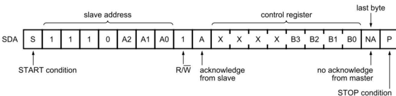
Figure 12. Read Control Register
