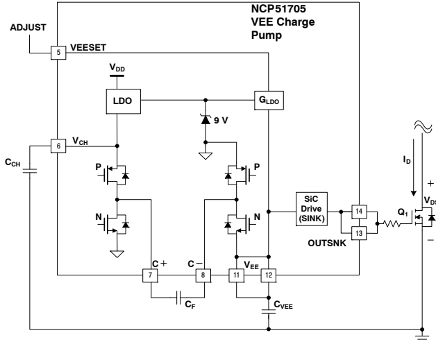
Figure 37. NCP51705 V_{EE} Charge Pump
