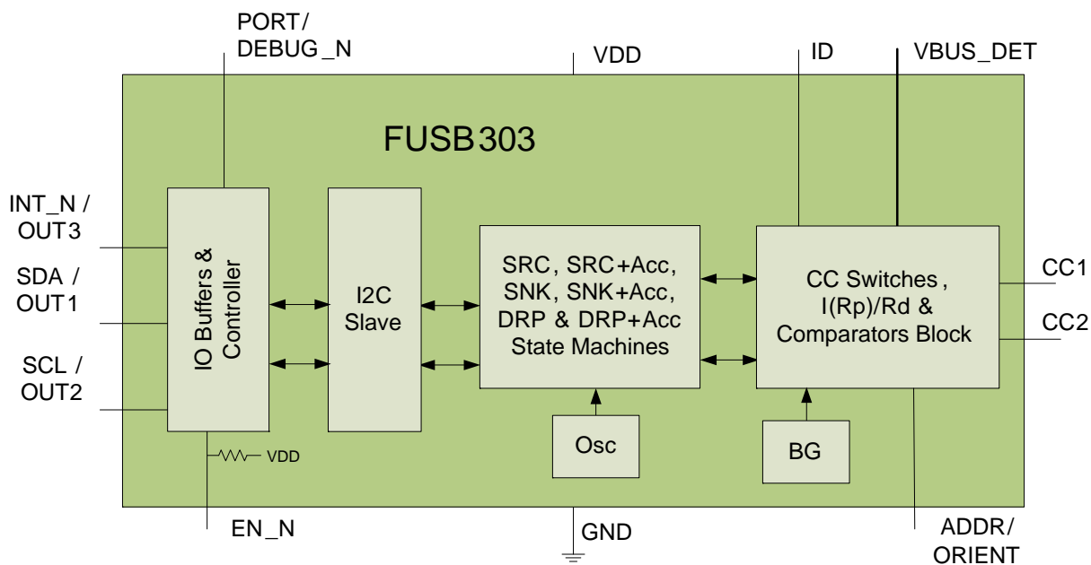
Figure 3. FUSB303 Block Diagram
