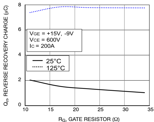
Figure 74. Typical Reverse Recovery Charge vs. R_G
