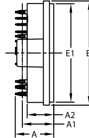
END VIEW
