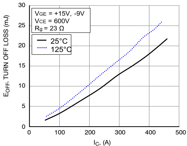
Figure 78. Typical Turn Off Loss vs. I_C
