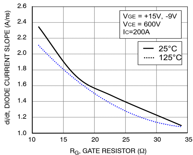
Figure 76. Typical di/dt vs. R_G
