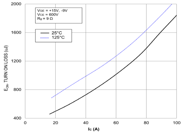
Figure 18. Typical Turn On Loss vs. I_C
