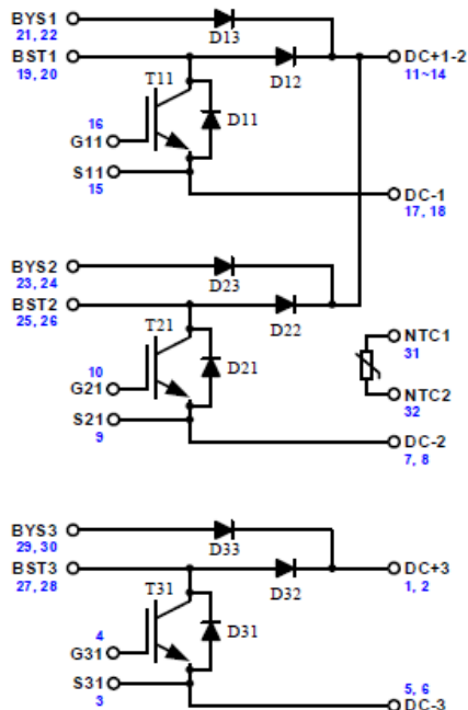
Figure 1. NXH240B120H3Q1 Schematic Diagram
