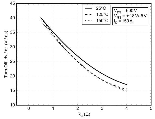
Figure 27. dv/dt OFF vs. R_G
