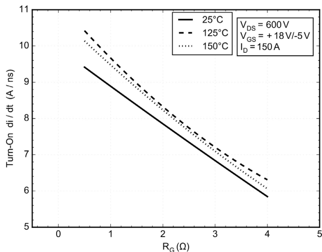
Figure 21. di/dt ON vs. RG
