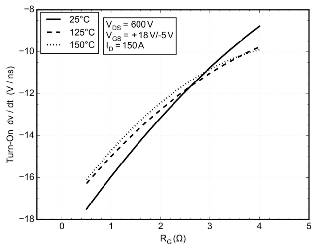
Figure 25. dv/dt ON vs. RG
