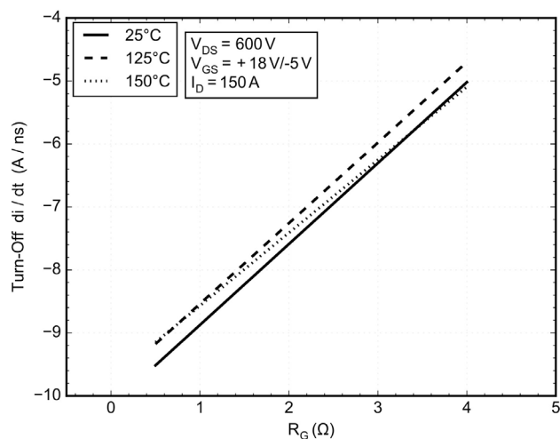
Figure 23. di/dt OFF vs. RG
