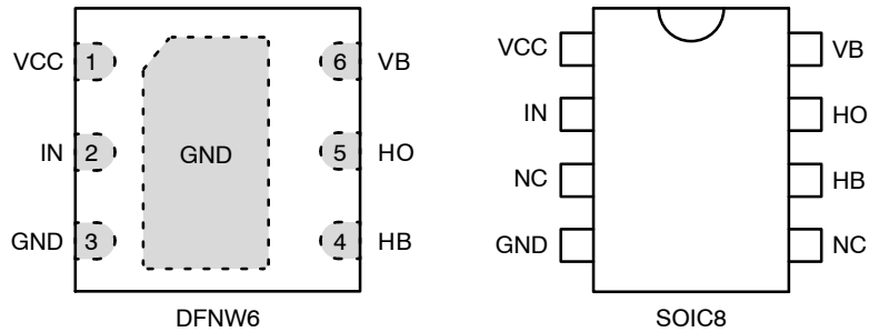
Figure 1. Pinouts
