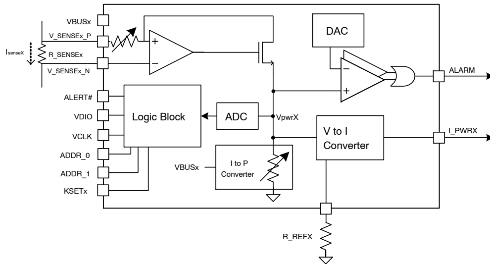
Figure 1. Block Diagram
