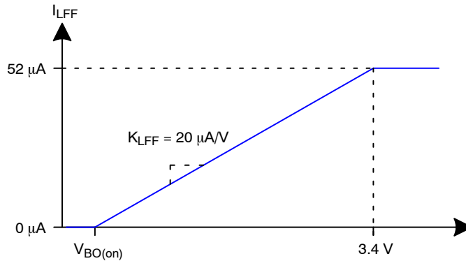
Figure 43. Transfer Function of the Line Feed Forward
