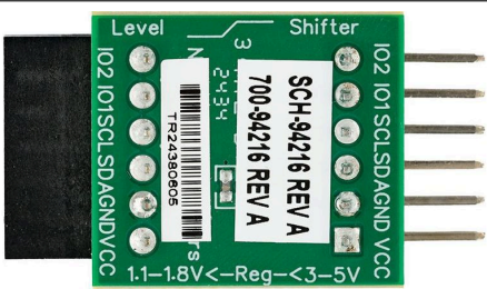
Figure 6. Level shifter - bottom view
