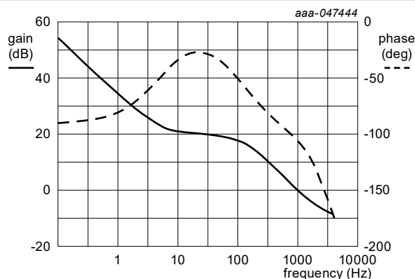
Figure 7. Transfer curve of digital PI controller
