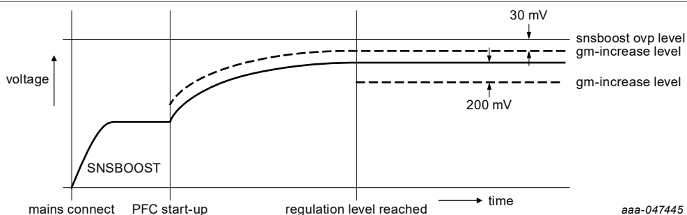
Figure 8. Gain increase limits
