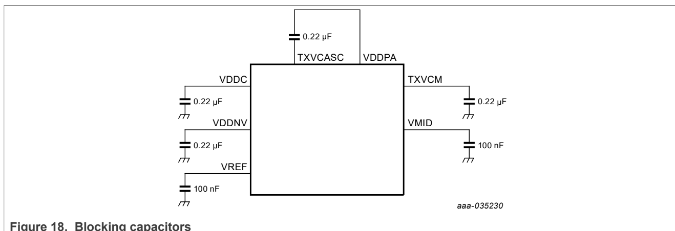
Figure 18. Blocking capacitors
