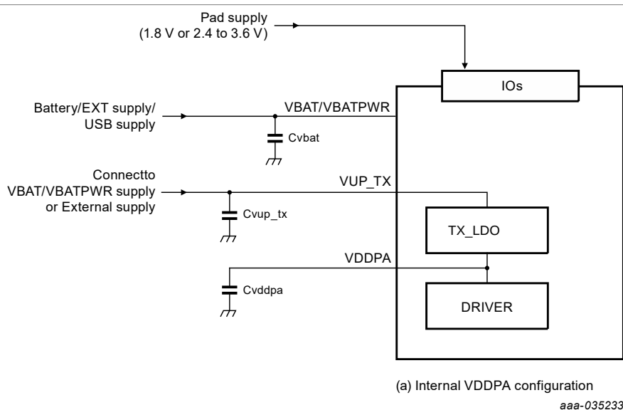
Figure 19. Transmitter supply
