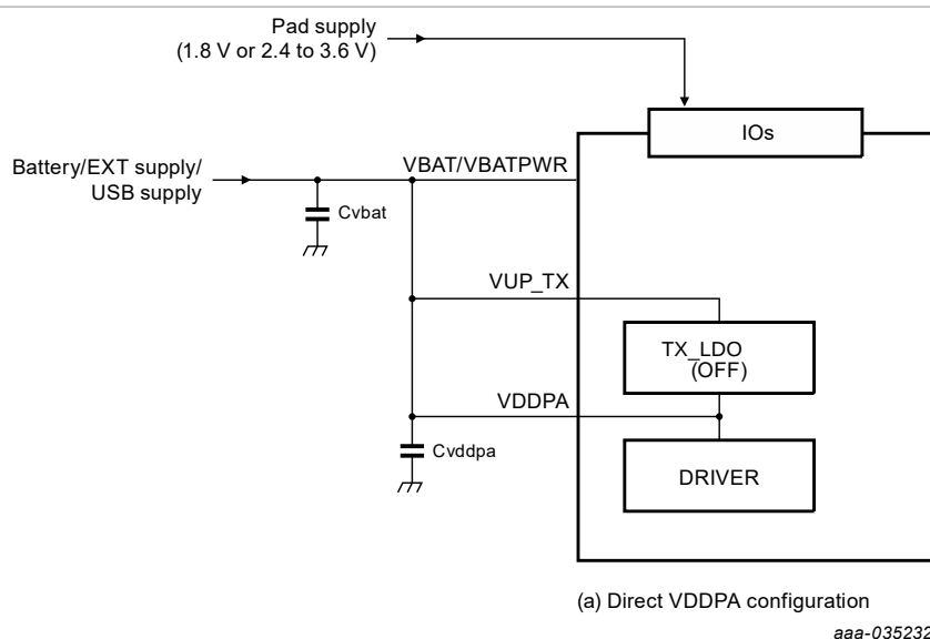
Figure 20. Direct transmitter supply
