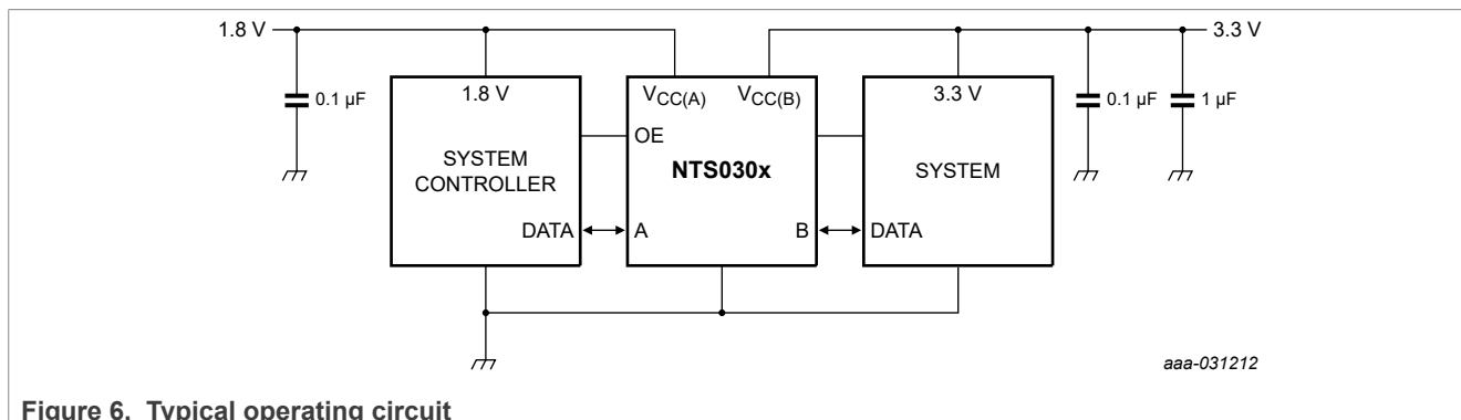
Figure 6. Typical operating circuit
