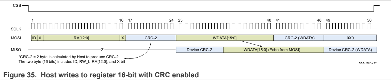
Figure 35. Host writes to register 16-bit with CRC enabled
