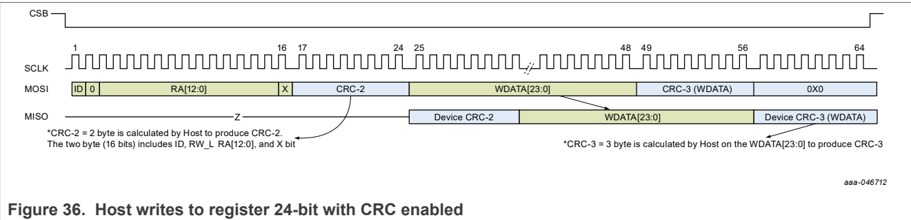
Figure 36. Host writes to register 24-bit with CRC enabled
