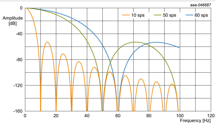
Figure 7. SINC Normal mode rejection vs frequency vs data rate
