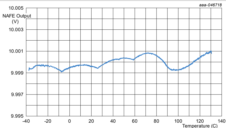
Figure 45. Temperature drift test
