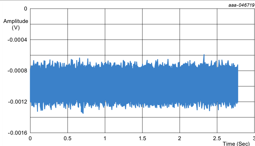
Figure 46. ADC conversion results
