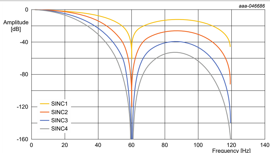
Figure 6. Second stage SINC filter transfer function
