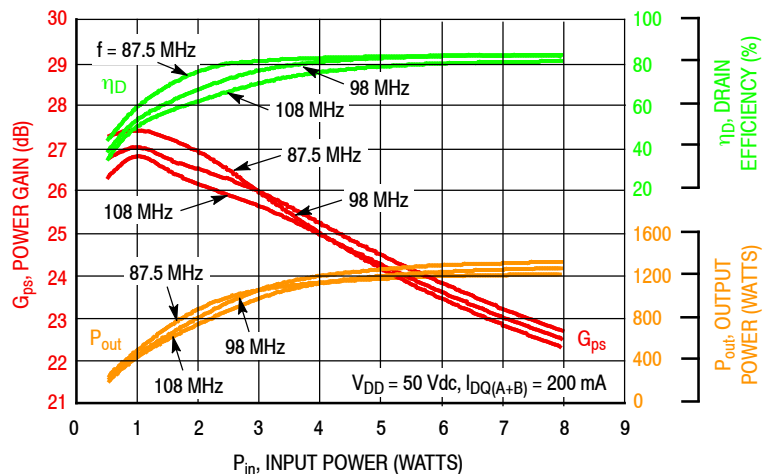
Figure 10. Power Gain, Drain Efficiency and CW Output Power versus Input Power and Frequency
