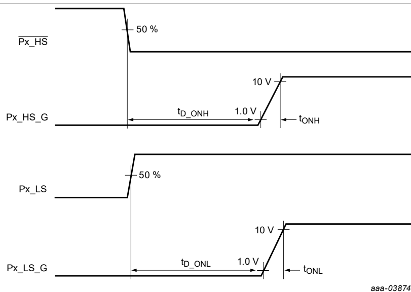
Figure 6. Driver turn-on time and turn-on delay
