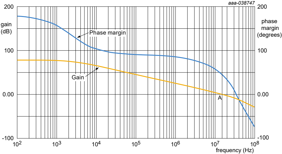
Figure 9. Typical amplifier open-loop gain and phase vs. frequency
