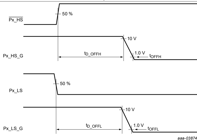
Figure 7. Driver turn-off time and turn-off delay
