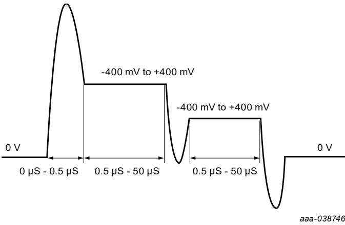
Figure 8. Current amplifier and input waveform ( V_{IN} voltage across R_{SENSE} )
