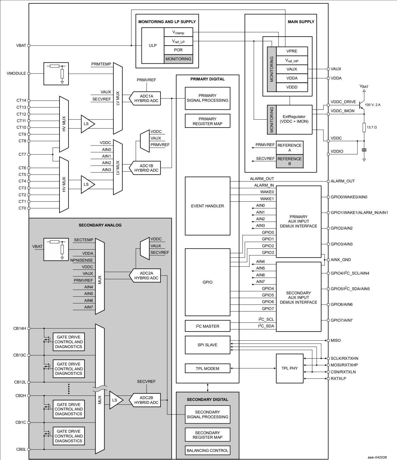
Figure 1. Block diagram
