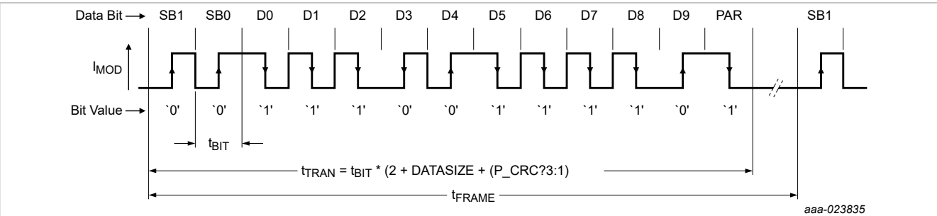
Figure 52. Example Manchester encoded data transfer – psi5-x10x
