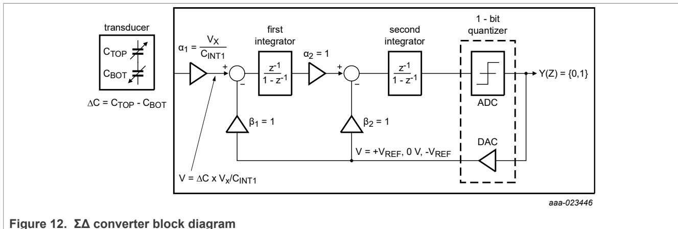
Figure 12. \Sigma\Delta converter block diagram
