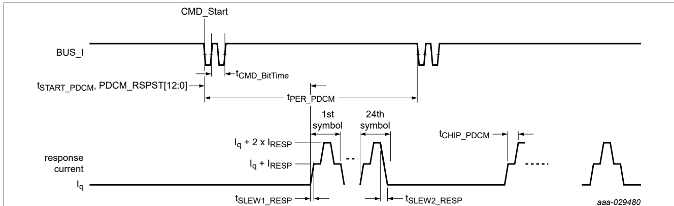
Figure 41. Periodic data collection mode timing diagram
