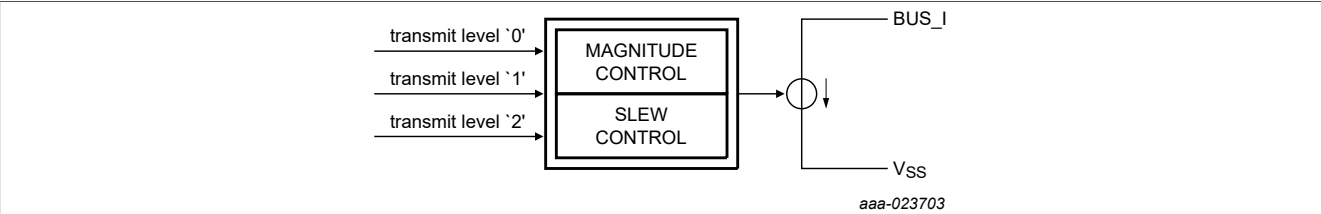
Figure 30. DSI3 transmitter block diagram
