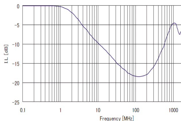
Insertion Loss Characteristics of 1259CM-0001
