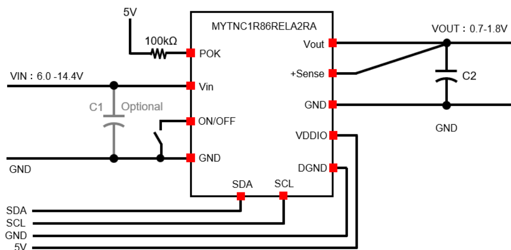
Figure 39. Application Schematic
