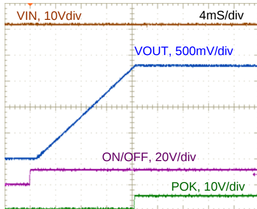
Figure 19. On/Off Enable wave form @+25°C (VIN=12V, VOUT=1.8V, IOUT=6A)
