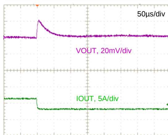
Figure 34. Step Load Transient Response (VIN=12V, VOUT=0.7V, COUT=200μF, IOUT=6 to 3A, 1.0A/μs)
