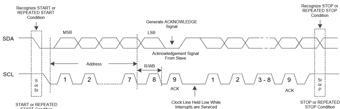
Figure 13. Bus Protocol
