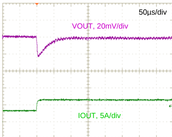
Figure 21. Step Load Transient Response (VIN=12V, VOUT=1.8V, COUT=200μF, IOUT=3 to 6A, 1.0A/μs)
