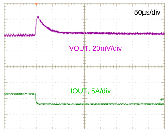
Figure 22. Step Load Transient Response (VIN=12V, VOUT=1.8V, COUT=200μF, IOUT=6 to 3A, 1.0A/μs)
