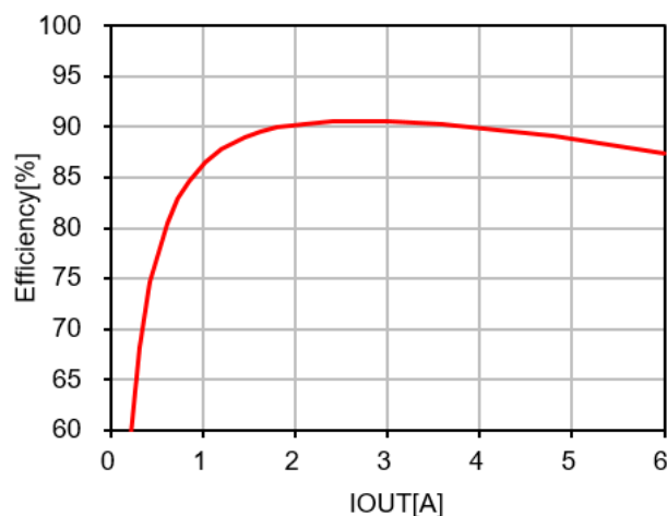
Figure 1. Efficiency Plot
