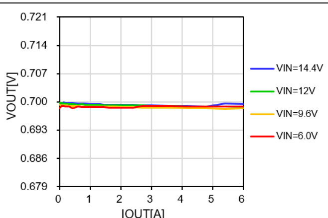
Figure 30. Vo vs. Load Current and Line Voltage @+25°C (VOUT= 0.7V)
