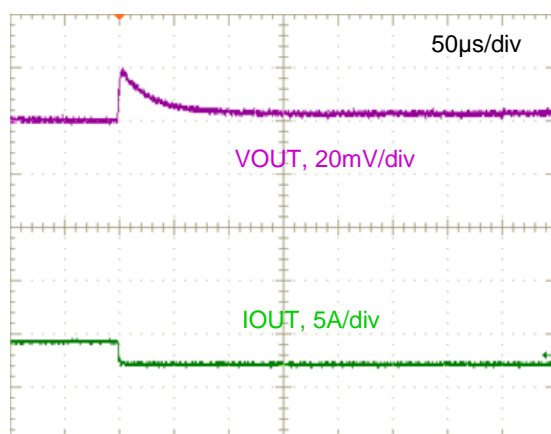
Figure 22. Step Load Transient Response (VIN=12V, VOUT=1.8V, COUT=200μF, IOUT=4 to 2A, 1.0A/μs)
