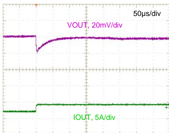
Figure 21. Step Load Transient Response (VIN=12V, VOUT=1.8V, COUT=200μF, IOUT=2 to 4A, 1.0A/μs)
