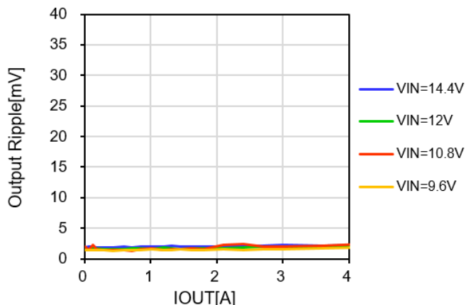
Figure 20. Output Ripple and Noise @+25°C (VOUT=1.8V, COUT=200μF, ScopeBW=20MHz)
