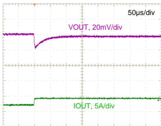
Figure 33. Step Load Transient Response (VIN=12V, VOUT=0.7V, COUT=200μF, IOUT=2 to 4A, 1.0A/μs)
