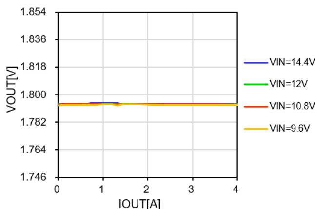
Figure 18. Vo vs. Load Current and Line Voltage @+25°C (VOUT=1.8V)
