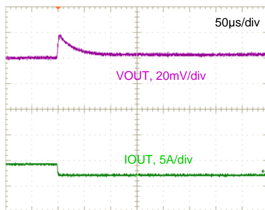
Figure 34. Step Load Transient Response (VIN=12V, VOUT=0.7V, COUT=200μF, IOUT=4 to 2A, 1.0A/μs)
