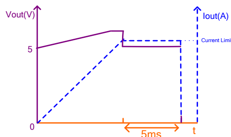
Figure 6: Over-Current Limit
