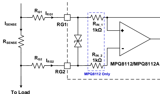
Figure 5: Back-to-Back Diodes
