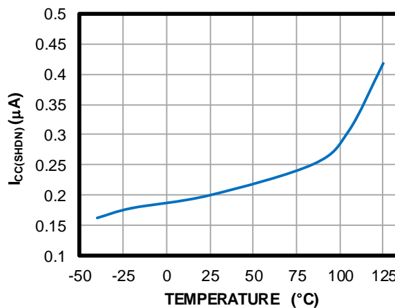
V5 Shutdown Supply Current vs. Temperature
