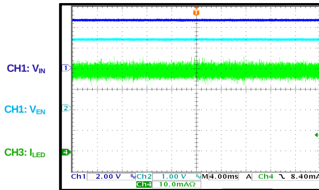
Analog Dimming 2.5mA/string
