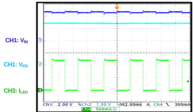
PWM Dimming PWM duty = 50%
