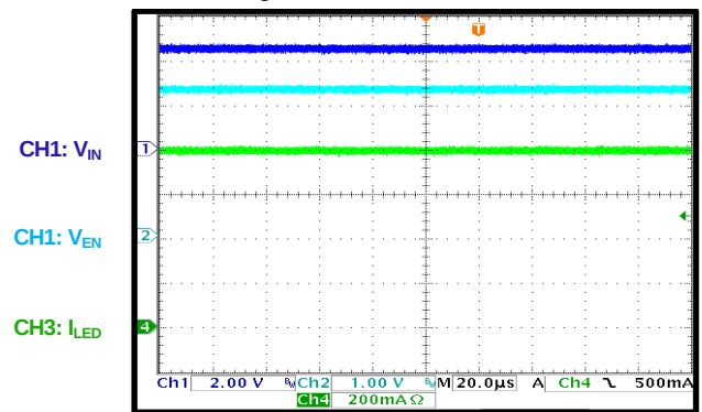
Analog Dimming 50mA/string
