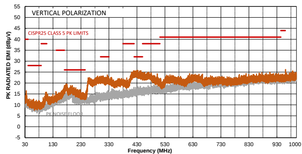
CISPR25 Class 5 Peak Radiated Emissions Vertical, 30MHz to 1GHz
