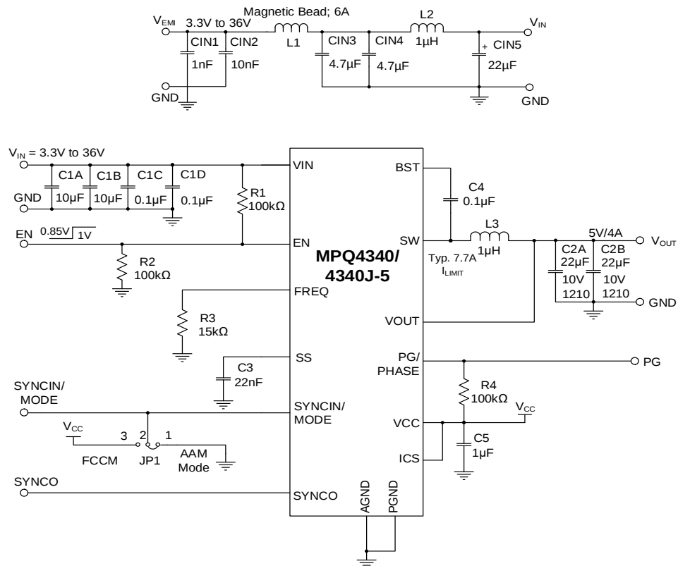
Figure 15: Typical Application Circuit (1-Phase, V_{OUT} = 5V , f_{sw} = 2.2MHz with EMI Filter)
